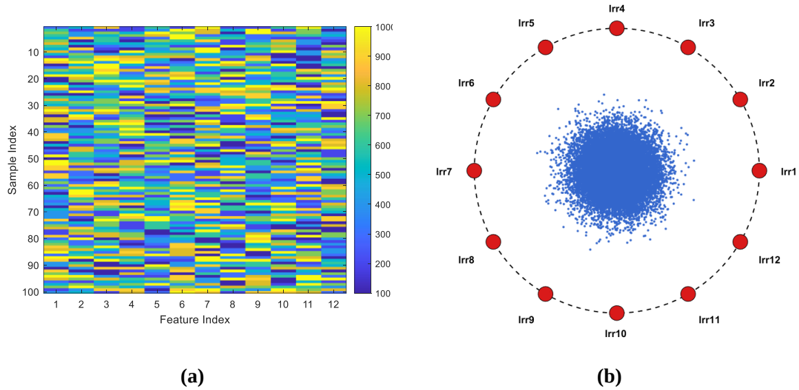
Figure 3. (a) Heatmap of 100 samples, (b) Inter-feature balance and sample mapping for 30000 samples
