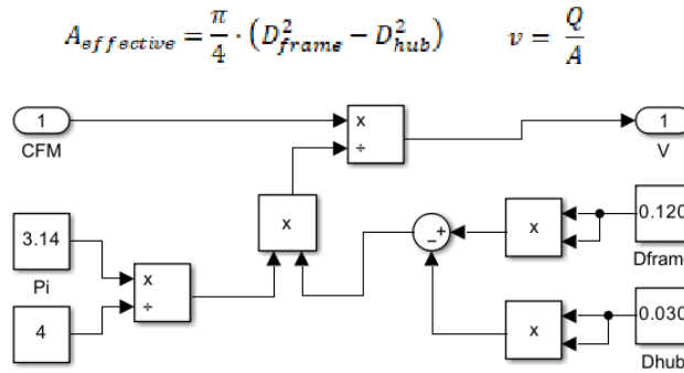
Figure 4. Subsystem for Calculating Airspeed from Air Volume Flow Rate
