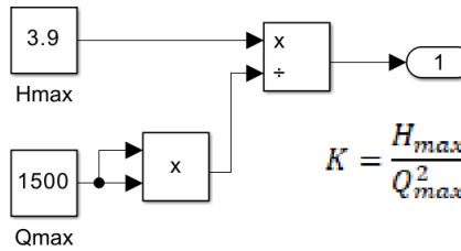
Figure 4. Subsystem for Calculating the K constant
