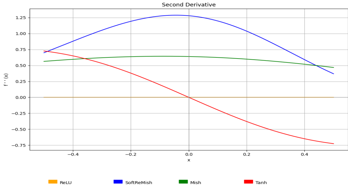
Figure 3. Second Derivatives of Activation Functions ReLU, Tanh, Mish and SoftReMish
