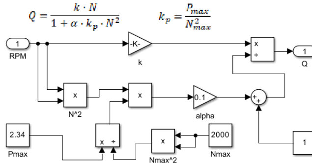
Figure 3. Subsystem for Calculating Airflow (CFM) from Fan Speed (RPM)
