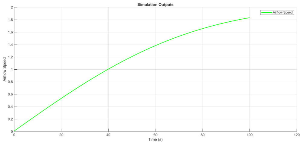
Figure 5. Scope Plot of Fan Airspeed (m/s) in Response to 2000 RPM Ramp Input Over 100 Steps
