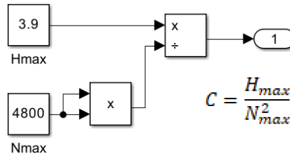
Figure 3. Subsystem for Calculating the C Constant
