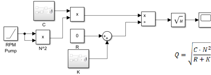
Figure 2. Simulink Model of the Pump System
