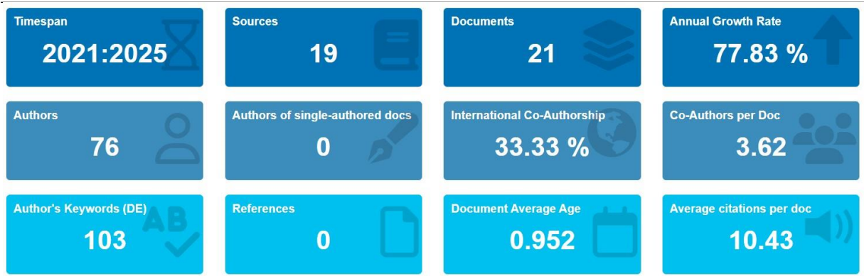
Figure 1. General Information
