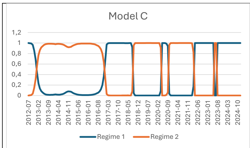
Figure 7: Model C
