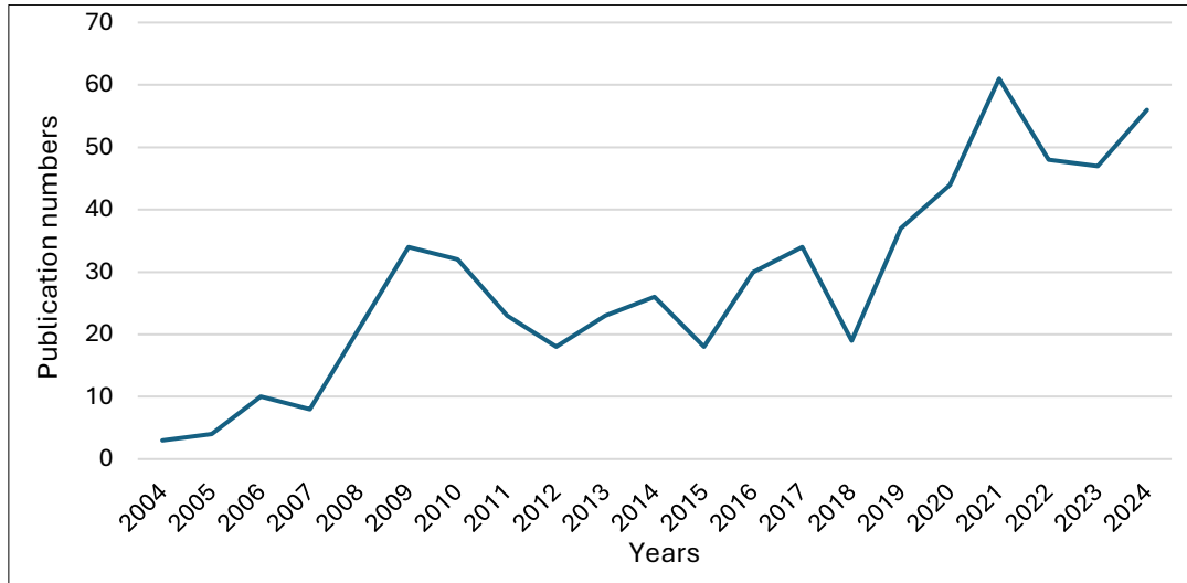
Figure 1. Publication years
