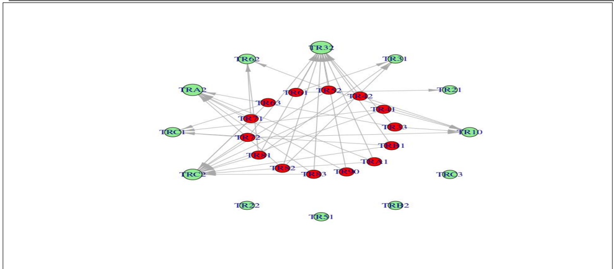
Figure 2. Network Graph
