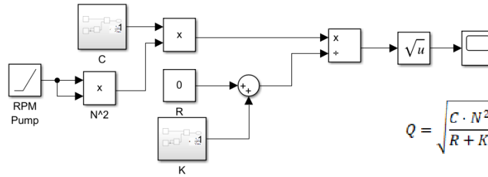
Figure 2. Simulink Model of the Pump System
