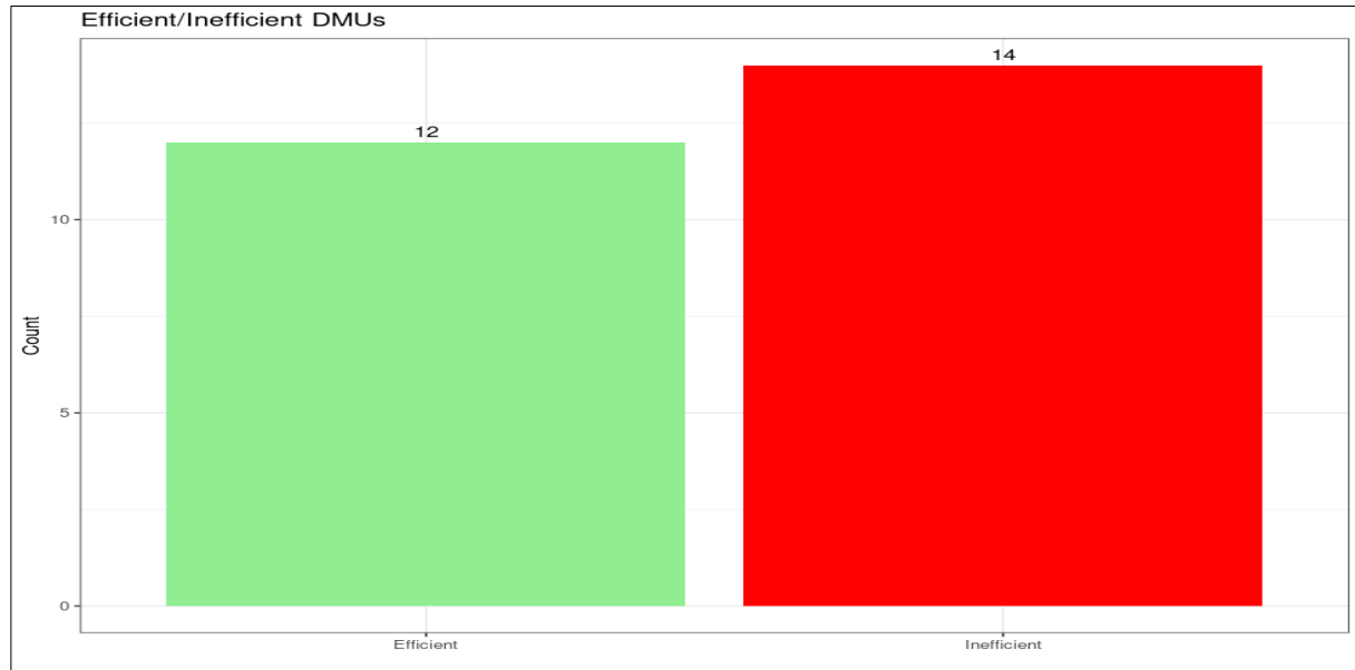
Figure 1. Efficiency Distribution
